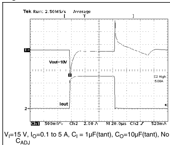
Figure 31. Load Transient
