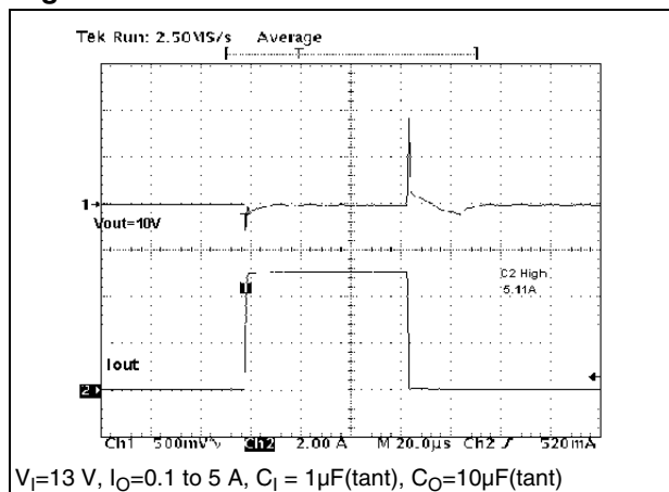
Figure 31. Load Transient
