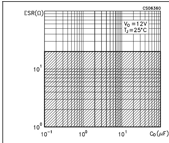
Figure 25. Stability
