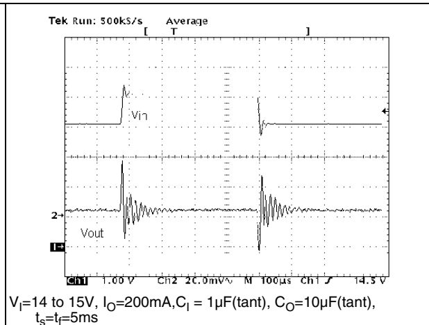
Figure 26. Line transient
